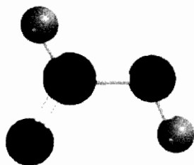
HCOOH
